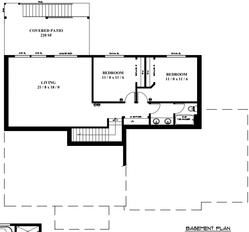
BASEMENT PLAN
